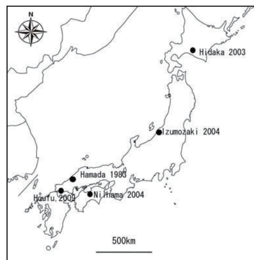
Fig.1 Locality map of the recent heavy rainfall-induced failures in Japan
